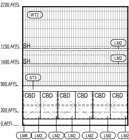
VILLAGE HEALTH & WELLNESS - CONSULT 1 ELEVATION 4 Scale 1: 50
