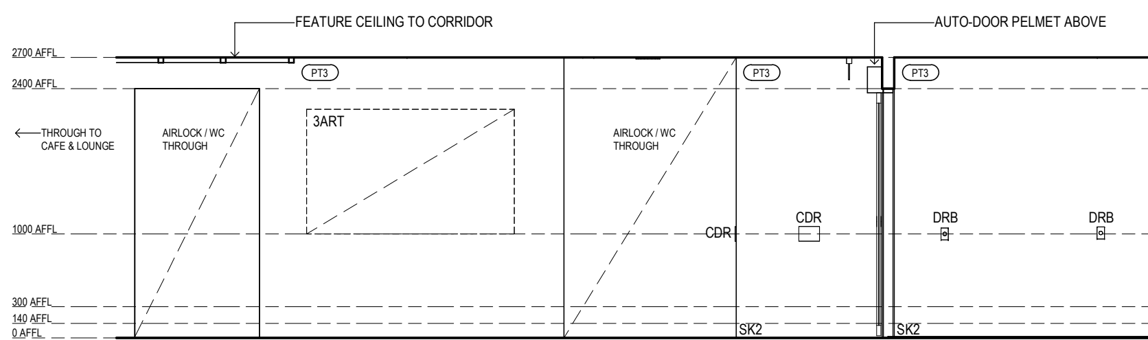
VILLAGE HEALTH & WELLNESS - AIRLOCK & CIRCULATION ELEVATION 1 Scale 1: 50
