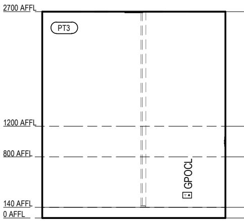
VILLAGE HEALTH & WELLNESS - CONSULT 1 ELEVATION 2 Scale 1: 50
