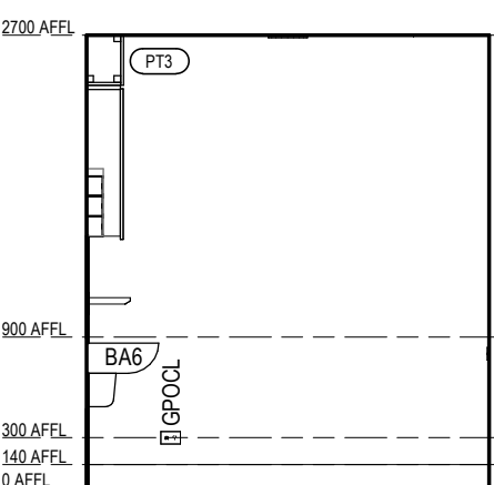
VILLAGE HEALTH & WELLNESS - CONSULT 2 ELEVATION 4 Scale 1: 50
