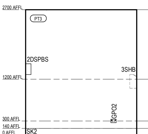
VILLAGE HEALTH & WELLNESS - CONSULT 2 ELEVATION 2 Scale 1: 50
